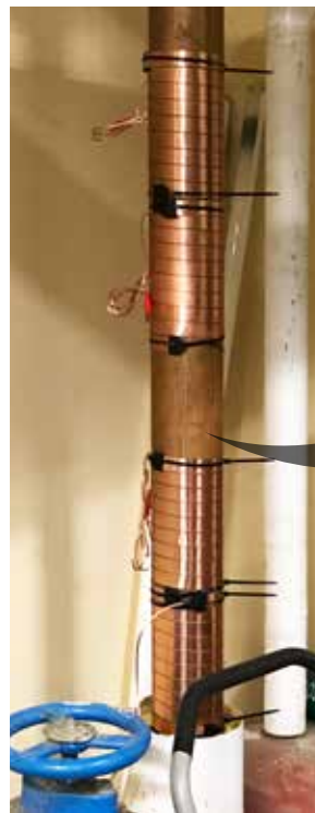
Step 1: Install the impulse bands
